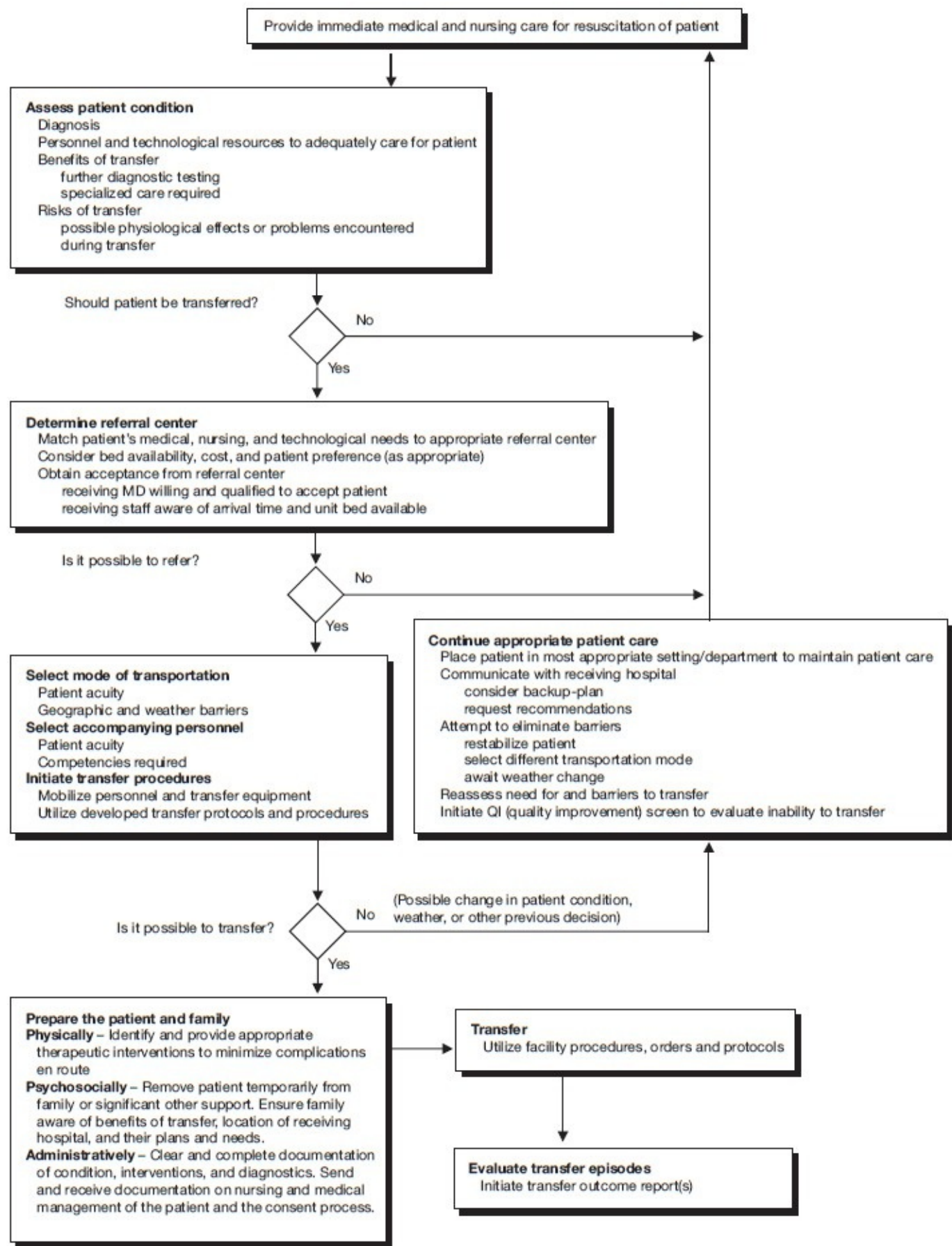
Figure 14-1. Transport Algorithm
