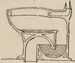
Fig. 60. Wash-out Closet.
