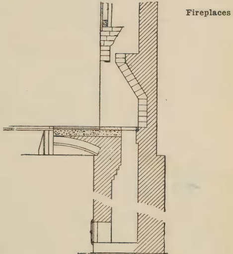
Fig. 15. Sectional View of a Well Constructed Fire-Place.
