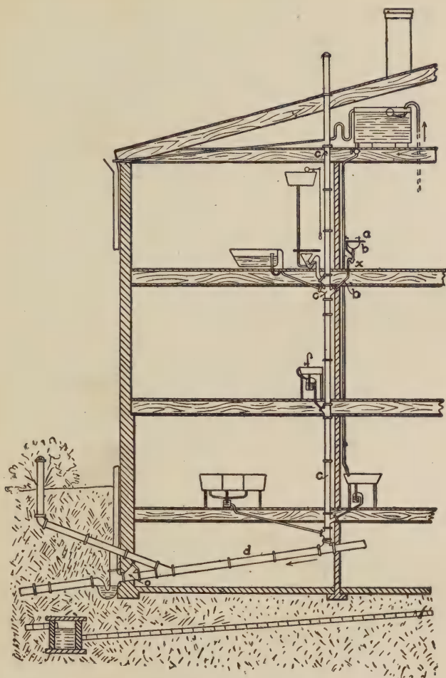
FIG. 51. HOUSE DRAINAGE SYSTEM.
