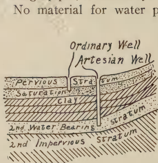
Fig. 36. Section Showing Ordinary and Artesian Wells.
