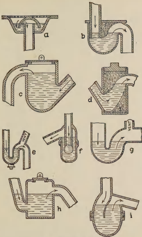
FIG. 52. STYLES OF TRAPS.
