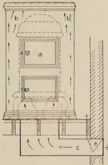
FIG. 18 A JACKETED STOVE.
