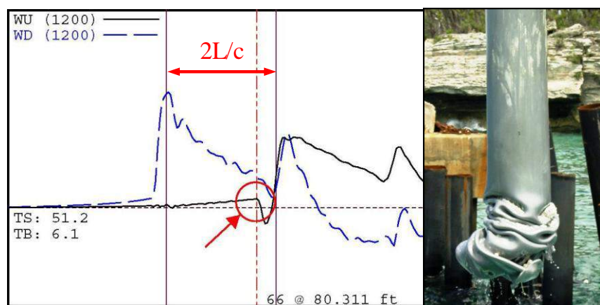
Fig. 9.15 Wave traces revealing damage to the pipe pile (later extracted). From Bullock (2012)
