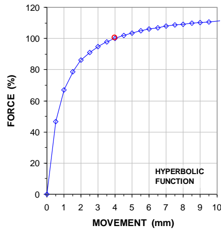
Fig. 8.13 Hyperbolic function for t-z shaft shear force vs. movement
