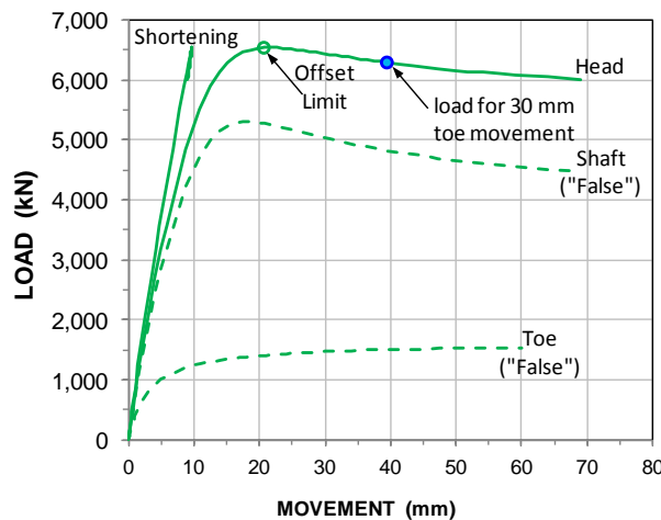
Fig. 8.18 Pile with residual load
