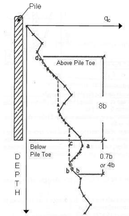
Fig. 7.9 Determining the influence zone for toe resistance (Schmertmann, 1978)
