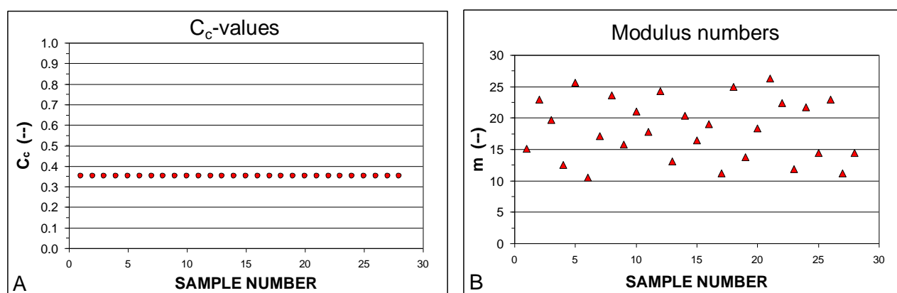
Fig. 3.6 "Selected" constant C_c -values, and converted via associated "selected" e_0 -values to "m"-values.
