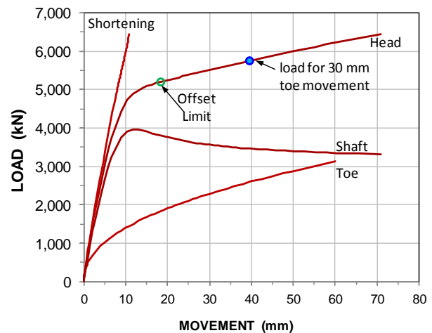
Fig. 8.19 Same pile without residual load
