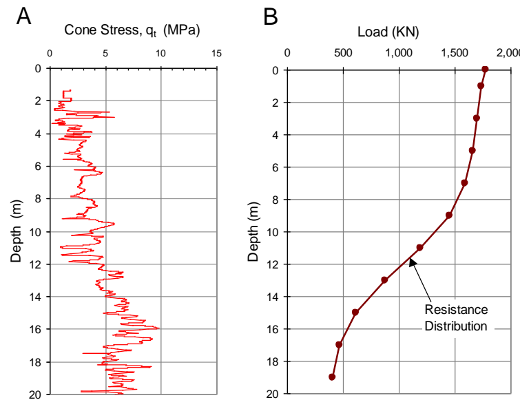
Fig. 8.35A CPT profile
