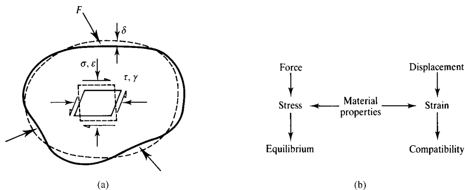
Figure 1.2 Principles of mechanics.
