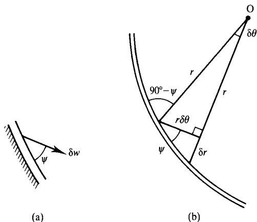
Figure 19.2 Geometry of a slip plane.
