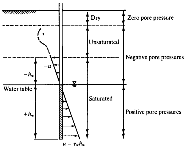
Figure 6.3 Pore pressures and suctions in the ground.
