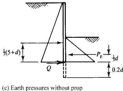
Figure 24.18 Analysis of a propped retaining wall – Examples 24.2 and 24.3.
