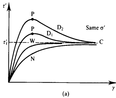
Figure 10.1 Initial states of samples at the same stress but different voids ratios.
