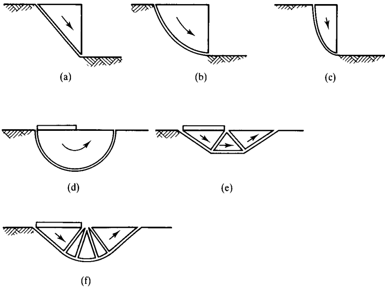
Figure 19.3 Compatible mechanisms.
