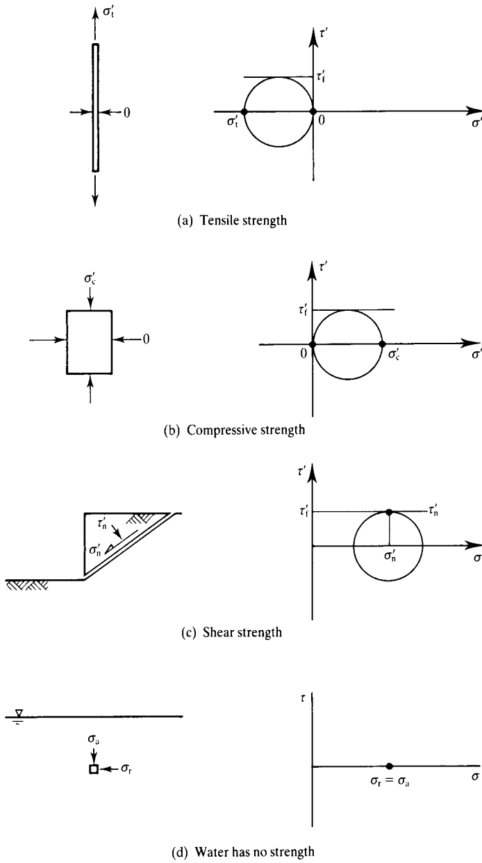
Figure 3.5 Strength of materials.
