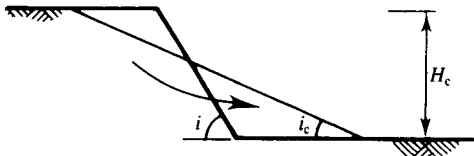
Figure 21.2 Simple slope failure.
