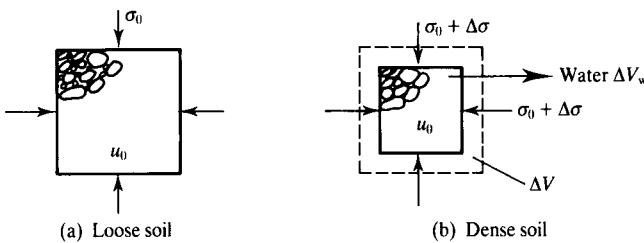
Figure 6.8 Volume changes in soil.
