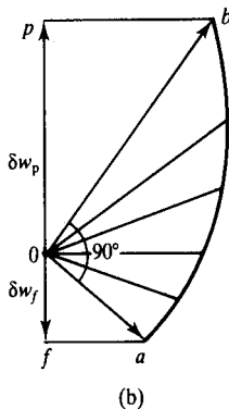
Figure 19.29 Mechanism of collapse for the foundation in Figure 19.26.
