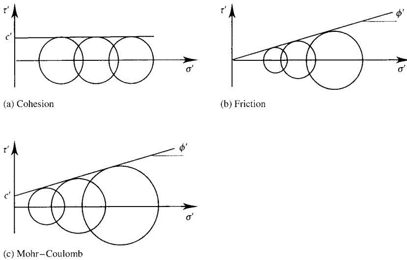
Figure 3.6 Failure criteria.
