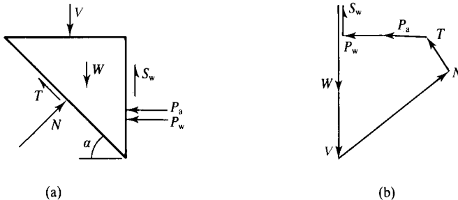
Figure 20.5 Coulomb wedge analysis for a rough wall for undrained loading.
