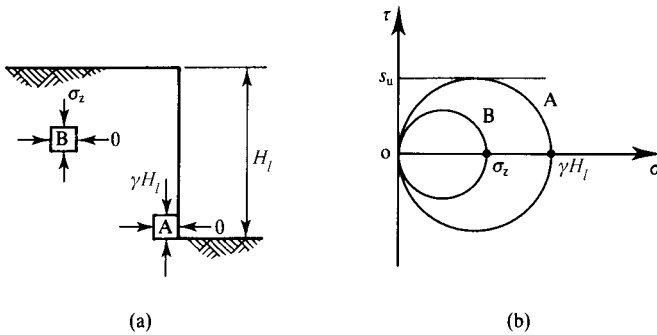
Figure 21.16 Equilibrium state of stress for a vertical cut slope for undrained loading.
