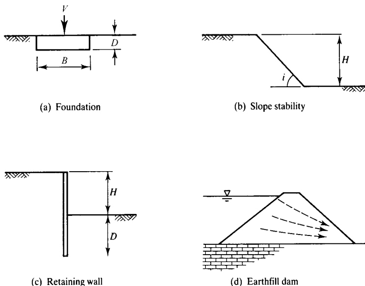
Figure 1.5 Geotechnical structures.
