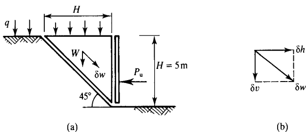
Figure 19.24 Mechanism of collapse for trench in Figure 19.23.
