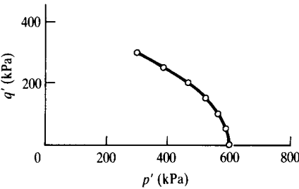
Figure 11.15 Undrained stress path – Example 11.3.
