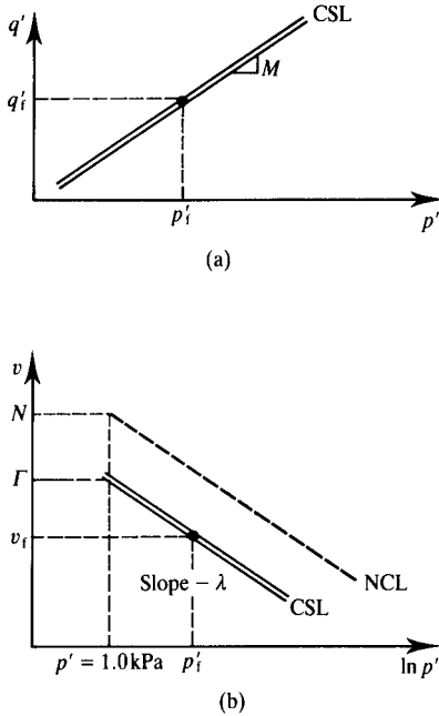
Figure 9.8 Critical state line for triaxial tests.
