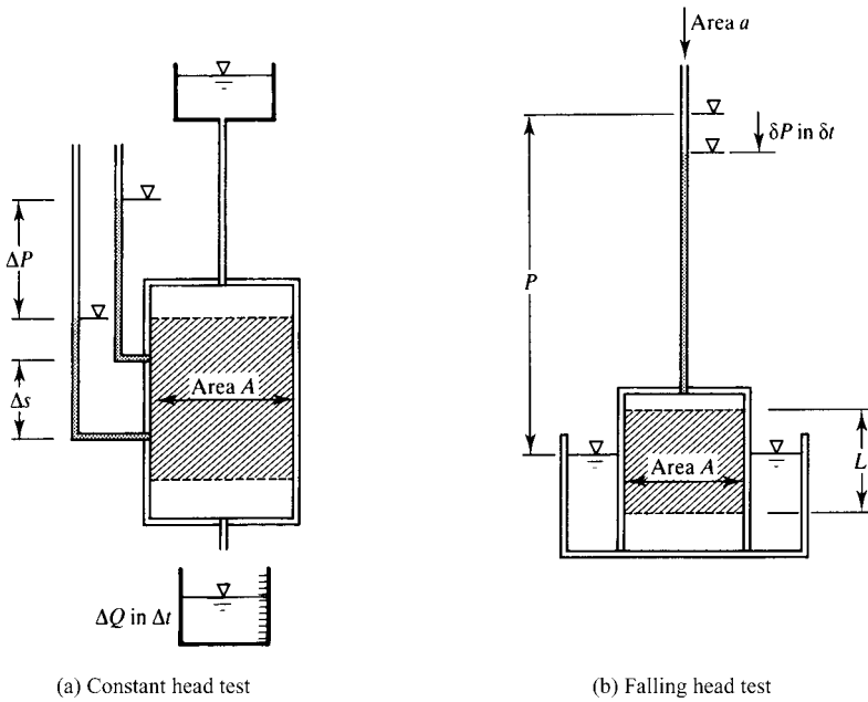
Figure 7.2 Permeameter tests.
