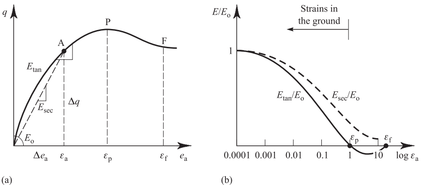
Figure 18.6 Tangent and secant moduli.
