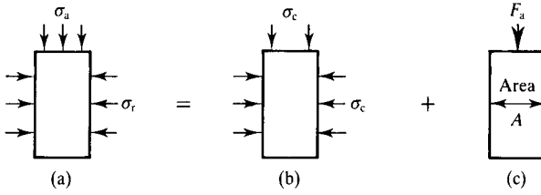
Figure 7.8 Stresses on a triaxial sample.
