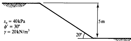
Figure 21.21 Stability of a simple slope – Examples 21.1 and 21.2.
