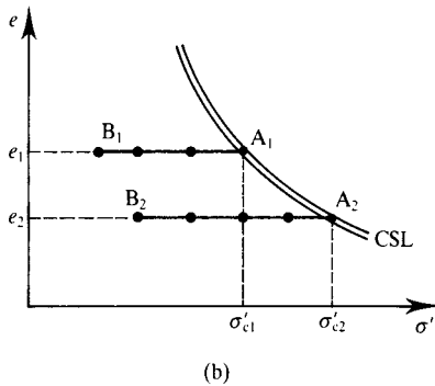
Figure 10.4 Mohr–Coulomb lines for peak states.
