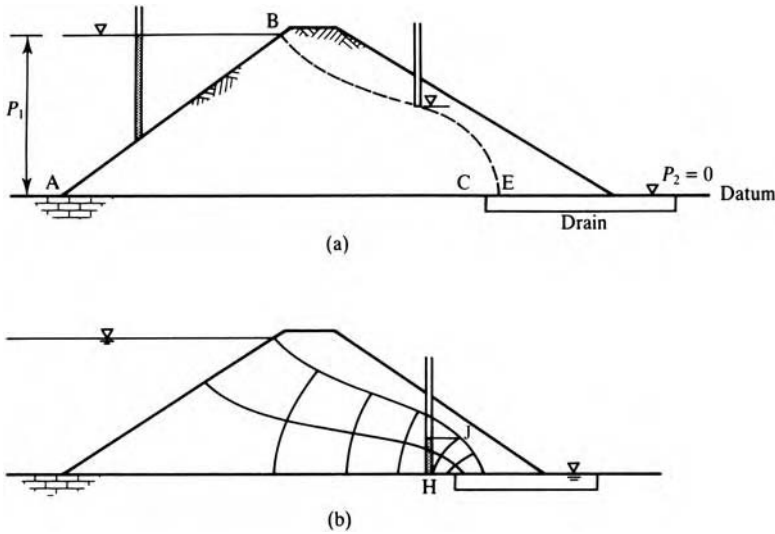
Figure 14.8 Flownet for steady state seepage through a dam.
