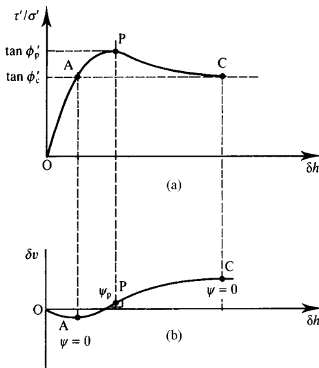
Figure 10.13 Shearing and dilation in shear tests.
