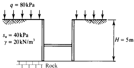
Figure 19.23 Trench supported by propped sheet piles.
