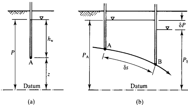
Figure 14.3 Pore pressure and potential.
