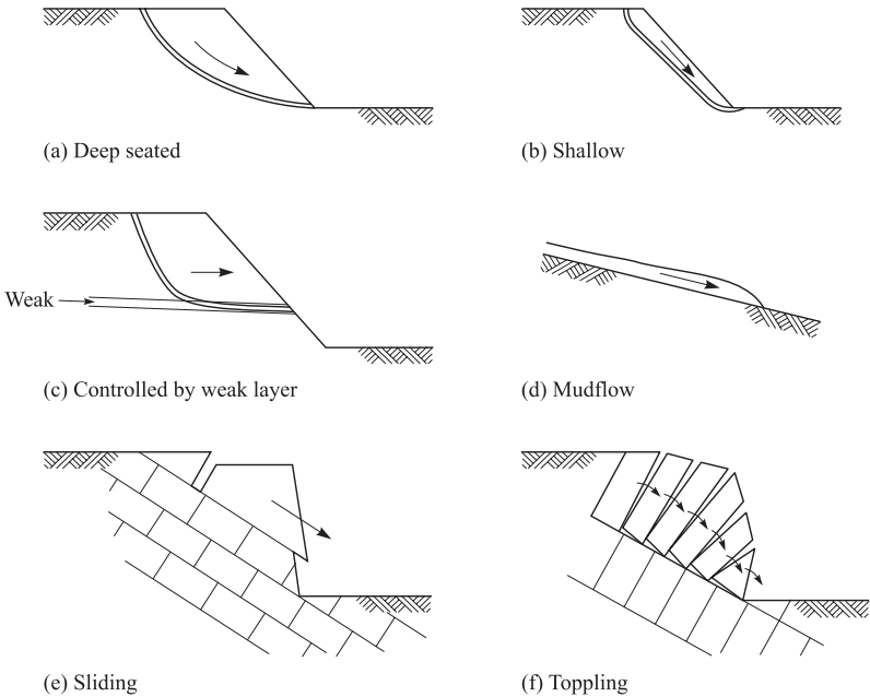
Figure 21.3 Types of slope failure.
