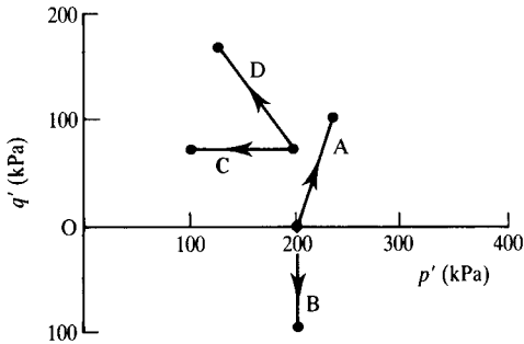
Figure 7.14 Stress paths – Example 7.5.
