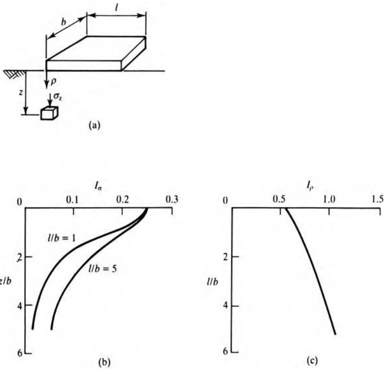
Figure 22.11 Influence factor for stresses and settlements below the corner of a rectangular foundation.
