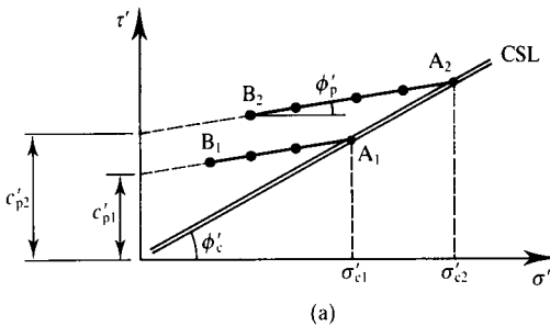
Figure 10.3 Region of peak states.
