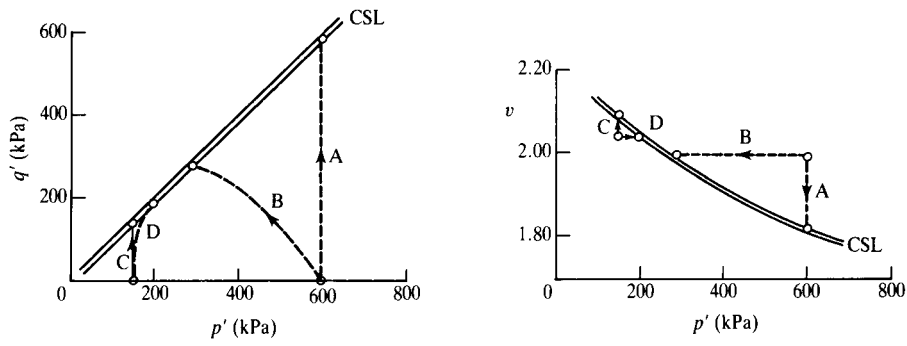
Figure 9.17 Results from tests on a soil – Example 9.2.
