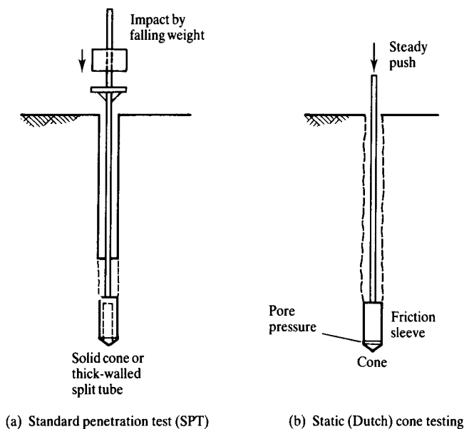
Figure 17.4 Probing tests (schematic).
