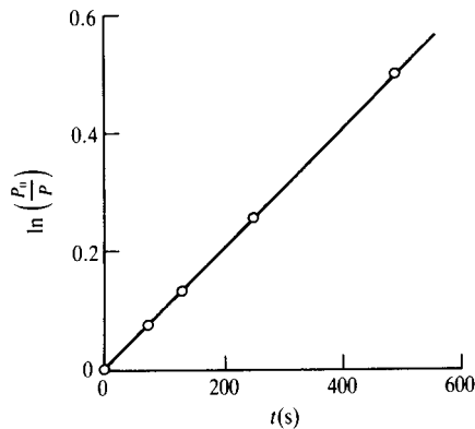
Figure 7.12 Results of falling head permeability test – Example 7.2.
