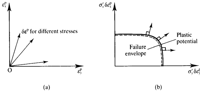
Figure 3.10 Plastic potential.
